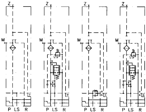
PSV5(6)-5 PSV5(6)/...-5 PSV5(6)S-5 PSV5(6)B/...-5
